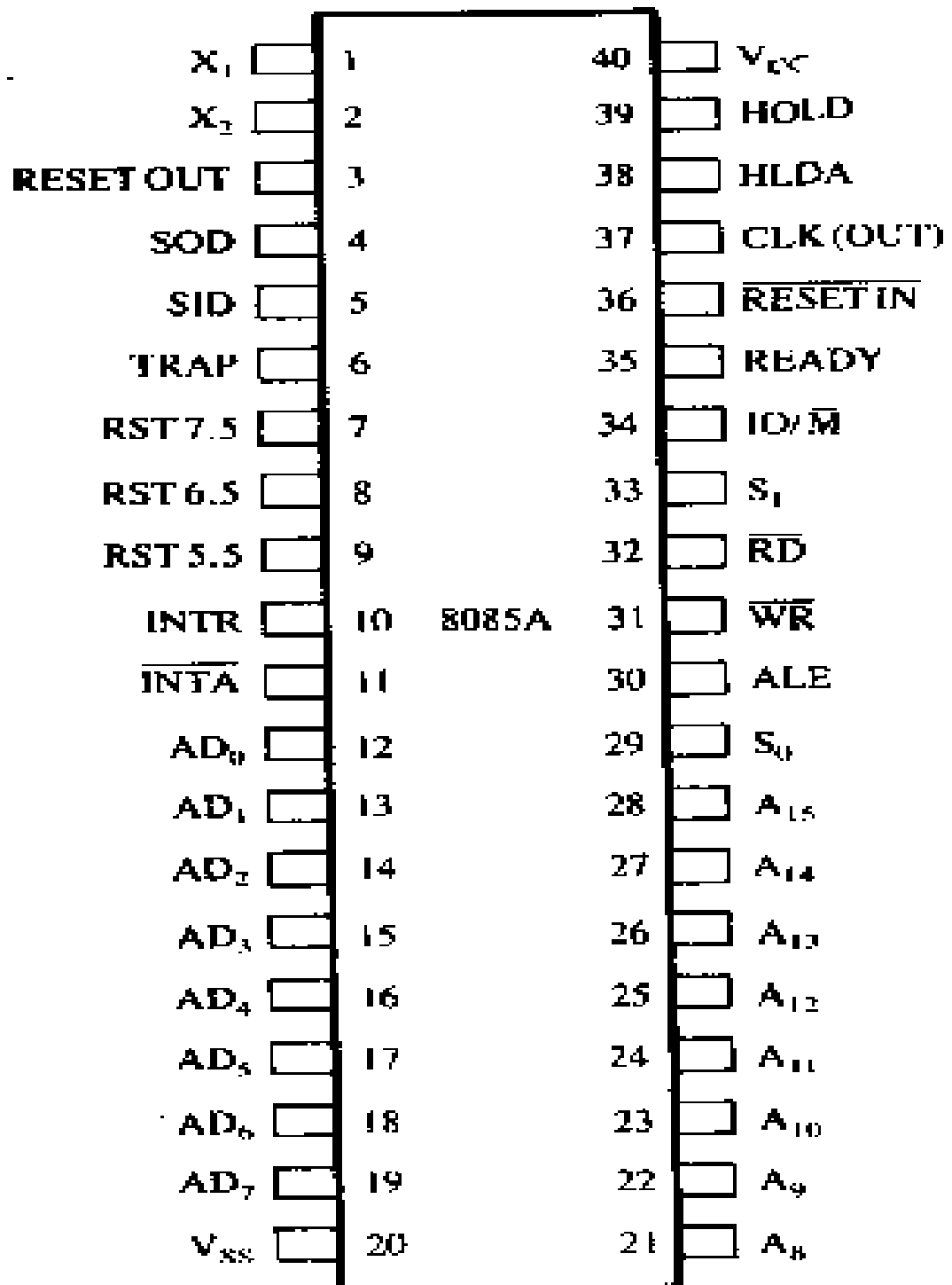
8085 Pinout
