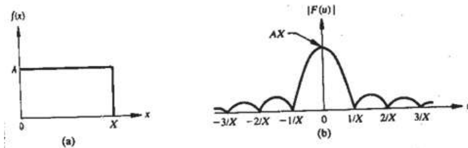
Fig 1 A simple function and its Fourier spectrum
