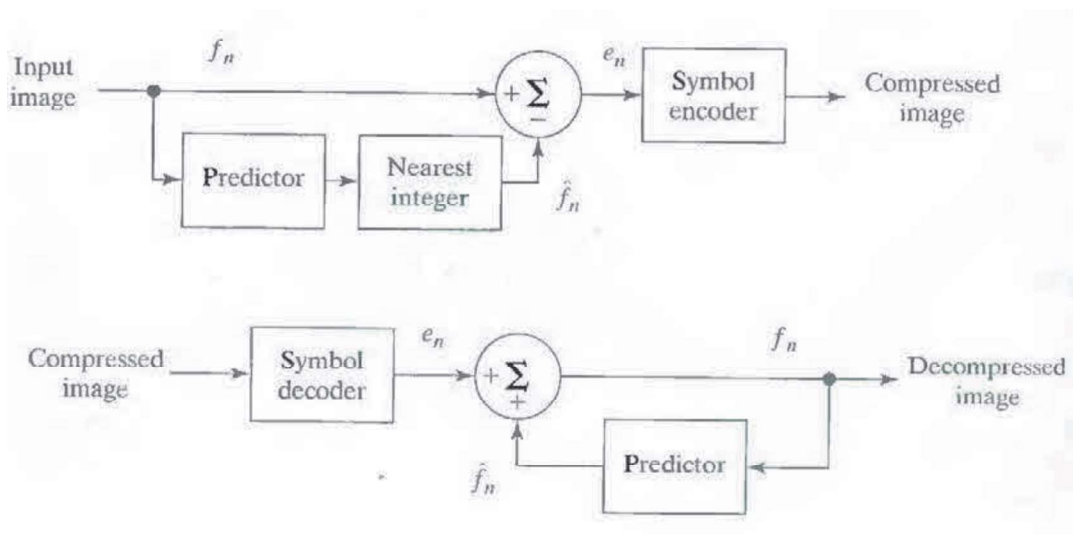
Fig.8.1 A lossless predictive coding model: (a) encoder; (b) decoder
