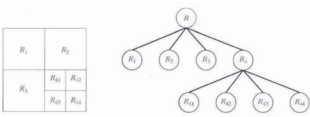
Fig. 7.3 (a) Partitioned image (b) Corresponding quadtree.
