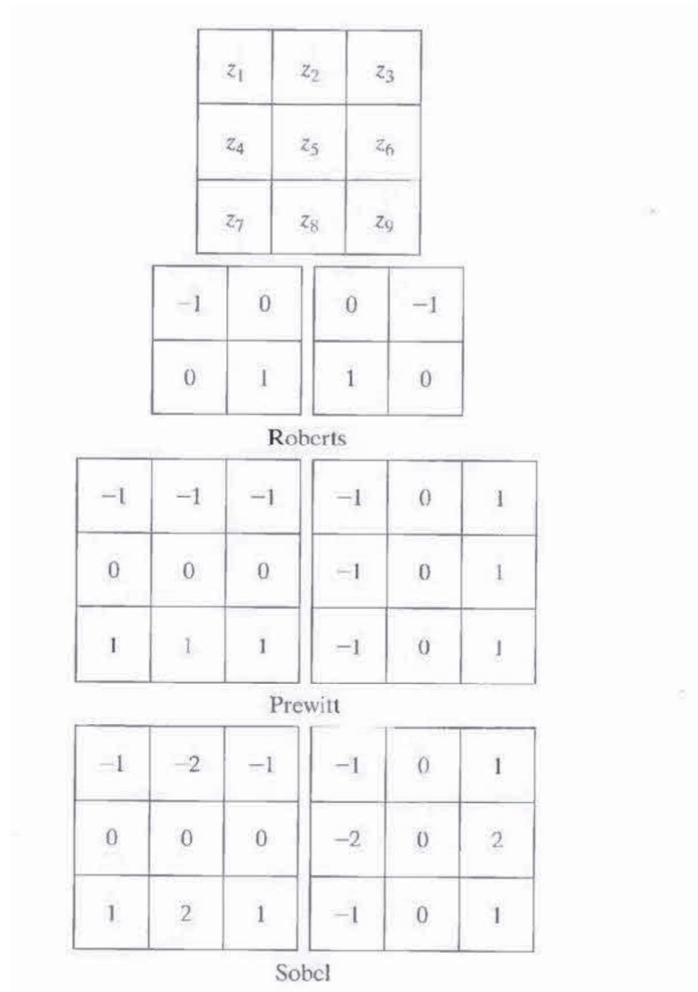
Fig.1.1 A 3 X 3 region of an image (the z's are gray-level values) and various masks used to compute the gradient at point labeled z_5 .
