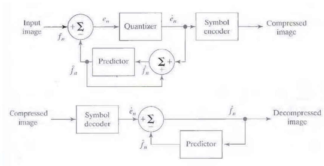
Fig. 9 A lossy predictive coding model: (a) encoder and (b) decoder.
