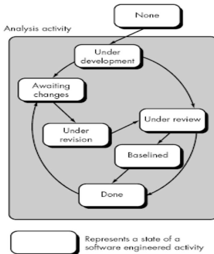
FIGURE: CONCURRENT DEVELOPMENT MODEL
