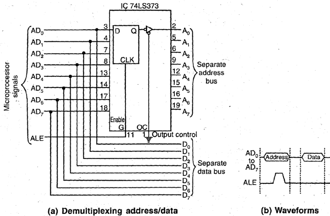
Fig 1.8 Demultiplexing of address and data bus
